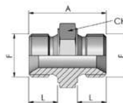
MALE X MALE ADAPTORS ADATTATORI MASCHIO X MASCHIO
