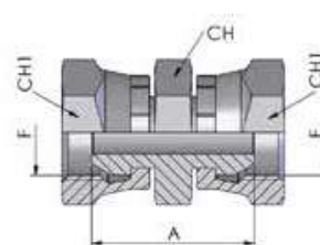
FEMALE X FEMALE ADAPTORS ADATTATORI FEMMINA X FEMMINA
