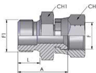
MALE X FEMALE ADAPTORS ADATTATORI MASCHIO X FEMMINA
