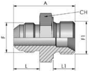
MALE X MALE ADAPTORS ADATTATORI MASCHIO X MASCHIO
